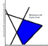
Linear Programming
